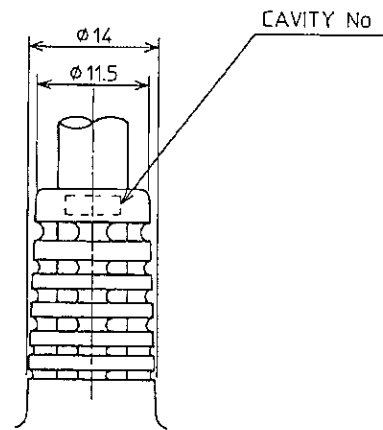
DETAIL OF STRAIN RELIEF 2/1
